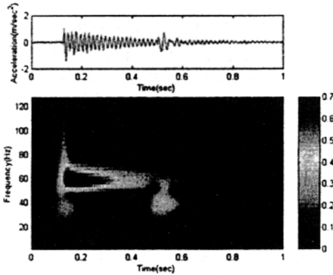
Fig. 1 CWT of the simulated impulse response
